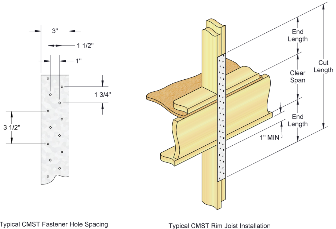
FIGURE 3—CMST COIL STRAP
