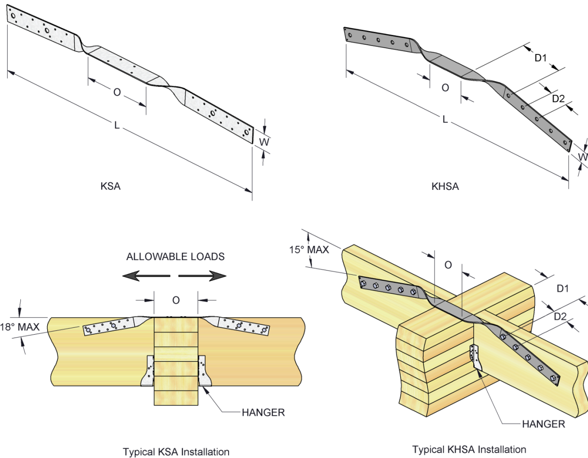
FIGURE 9—KSA & KHSA CONNECTOR STRAPS
