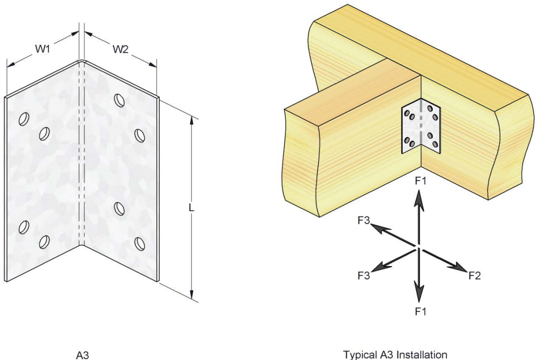
FIGURE 1—DIMENSIONS AND INSTALLATION OF A3 FRAMING ANGLE
