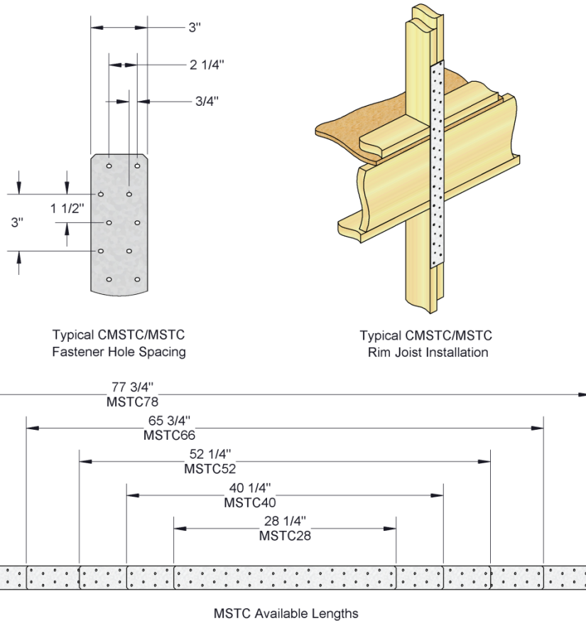
FIGURE 4—MSTC AND CMSTC STRAP TIE
