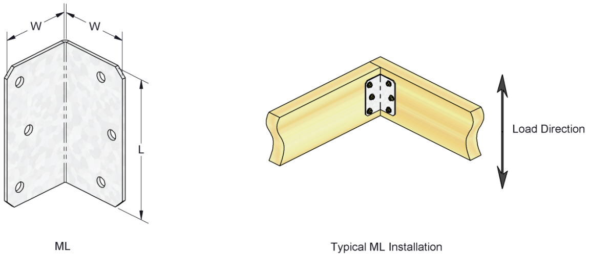
FIGURE 16—ML ANGLE CONNECTOR AND TYPICAL INSTALLATION DETAIL
