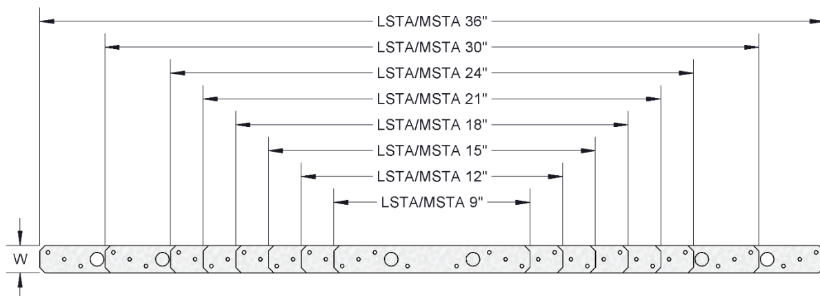
FIGURE 15—LSTA AND MSTA STRAP TIES
