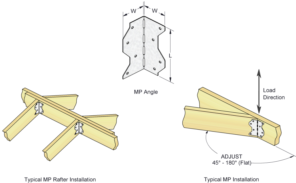
FIGURE 17—MP FRAMING ANGLE
