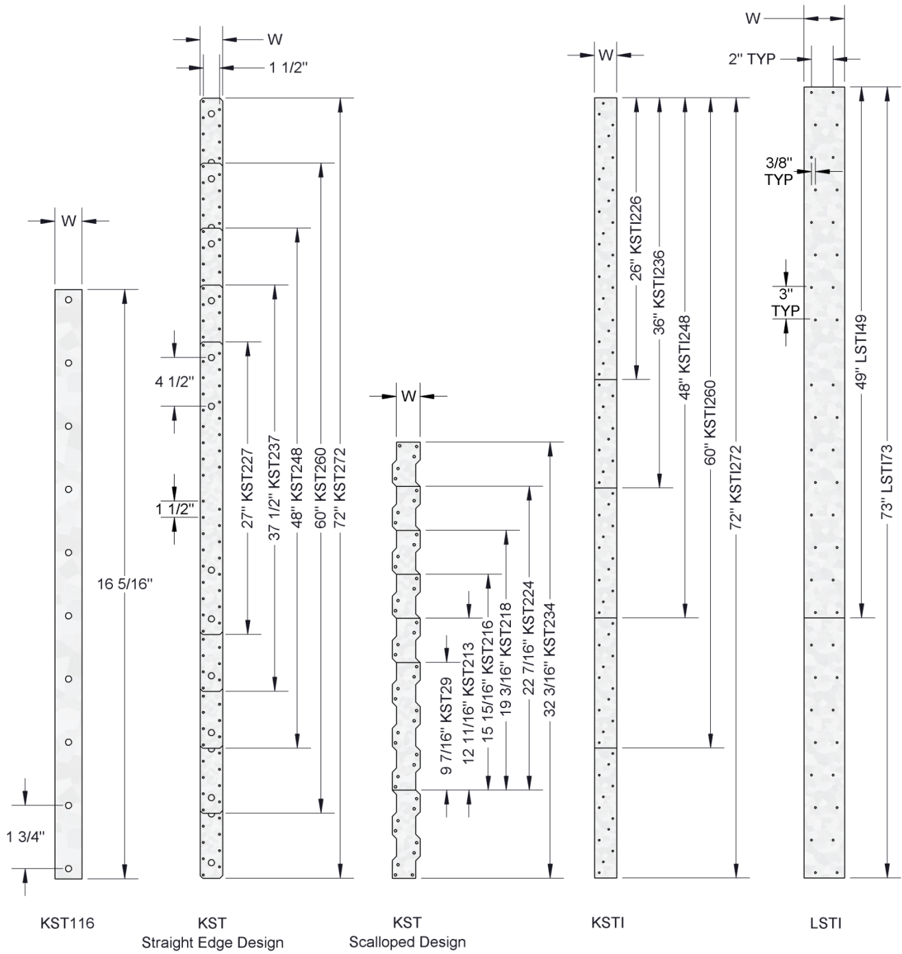
FIGURE 12—KST, KSTI AND LSTI STRAP TIES
