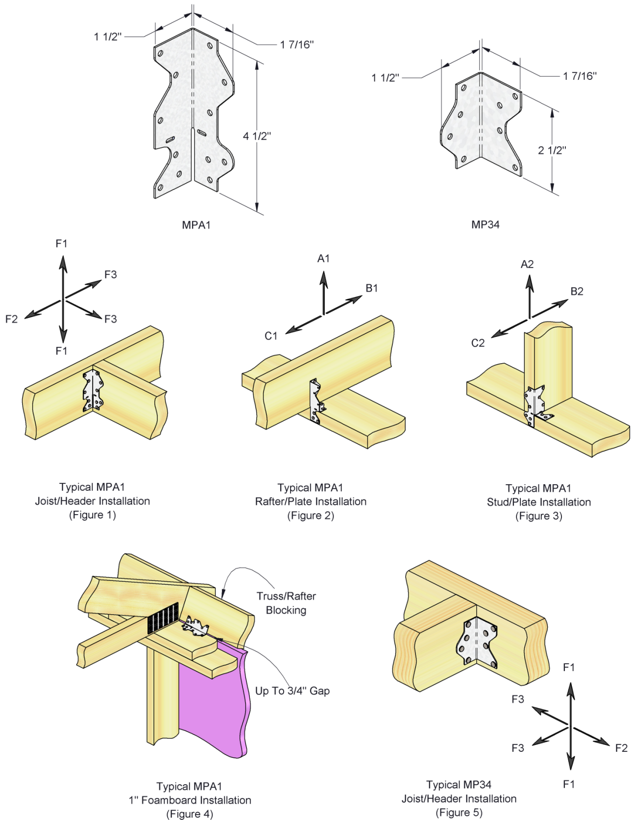
FIGURE 18—MP MULTI-PURPOSE FRAMING ANGLE
