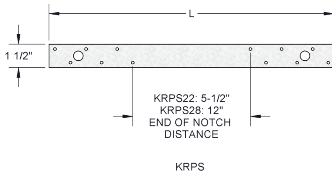
FIGURE 11—KRPS STRAP TIE AND TYPICAL INSTALLATION DETAIL
